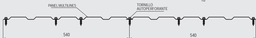
ENSAMBLE PANEL MULTILINES 110/10 T
