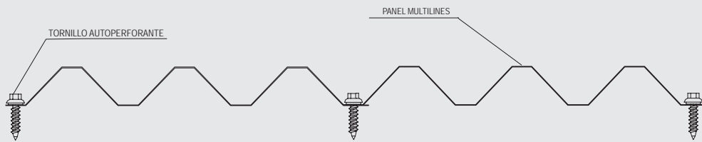
ENSAMBLE PANEL MULTILINES 90/30 T
