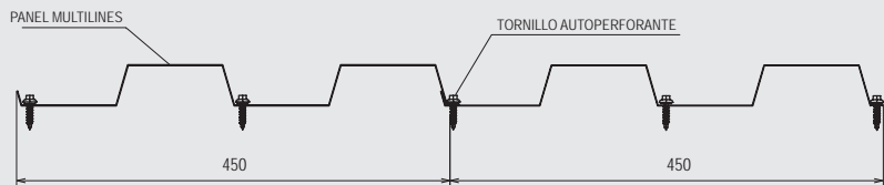
ENSAMBLE PANEL MULTILINES 225/45 C
