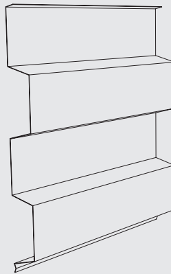
ENSAMBLE PANEL MULTILINES 225/45 C
